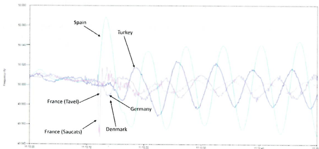
Figure 7: Frequency in different locations of SA CE at East-West mode oscillation on 1 st December 2016 (ENTSO-E analysis of CE inter-area oscillations of 1 st December)
