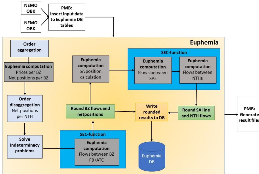
Figure 6: Calculation process
