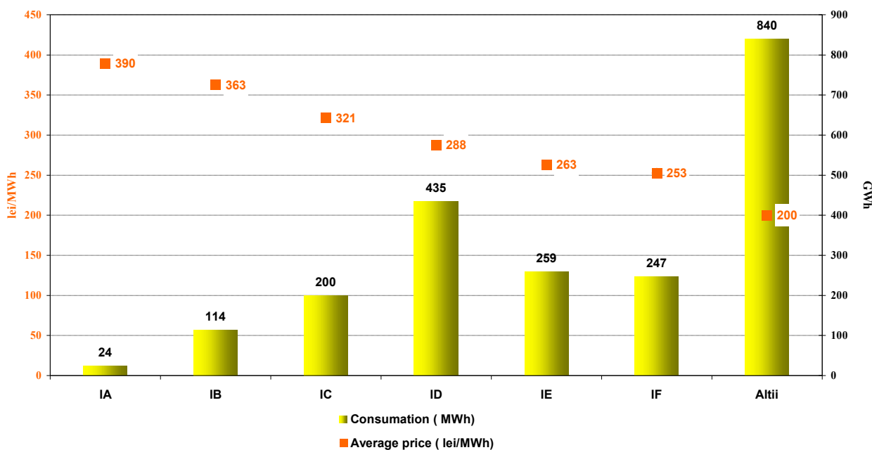
Average price and energy consumption on types of consumers applied on competitive market - July 2011 -
