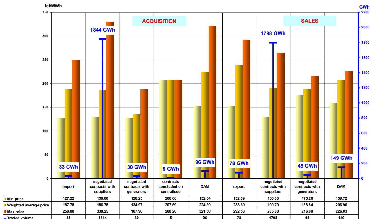
Transactions concluded by suppliers acting exclusively on WEM - JULY 2011 -
