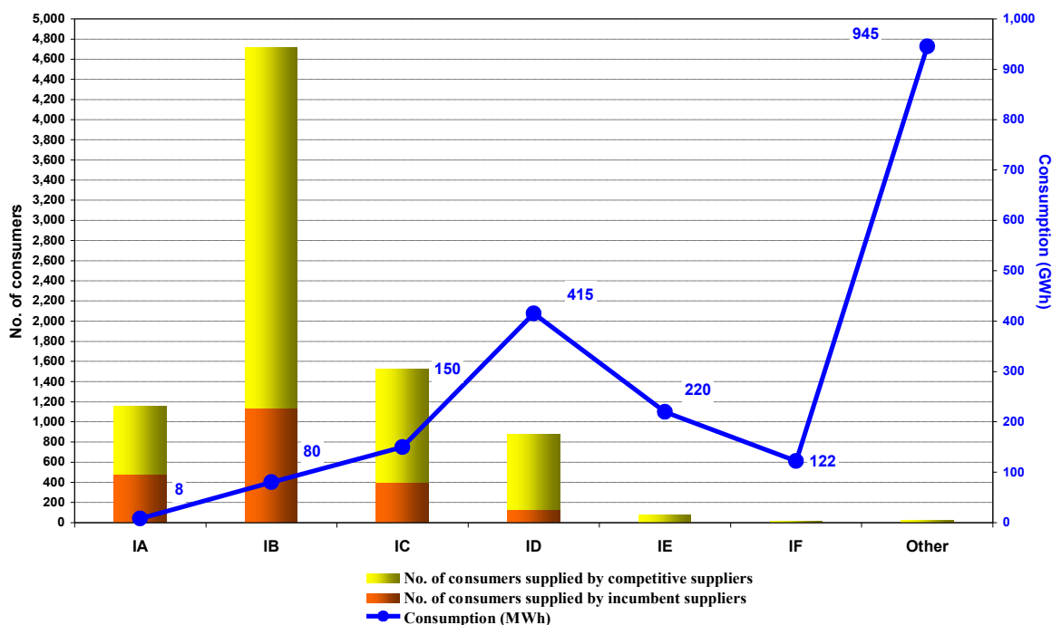
Number of consumers supplied on competitive market and the consumption of each category of consumers - July 2010 -
