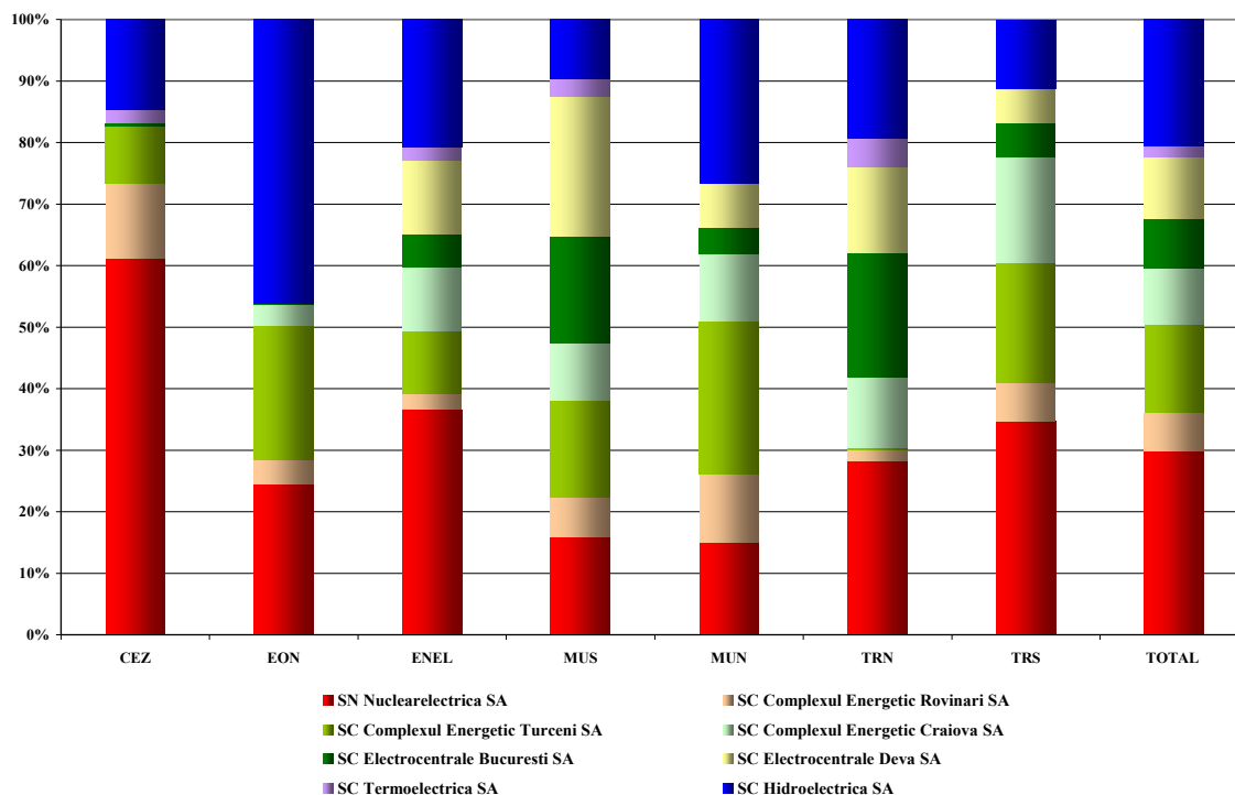
Electricity acquisition from main generators, on regulated contracts, of incumbent suppliers for delivering electricity to final consumers on regulated market July 2010
