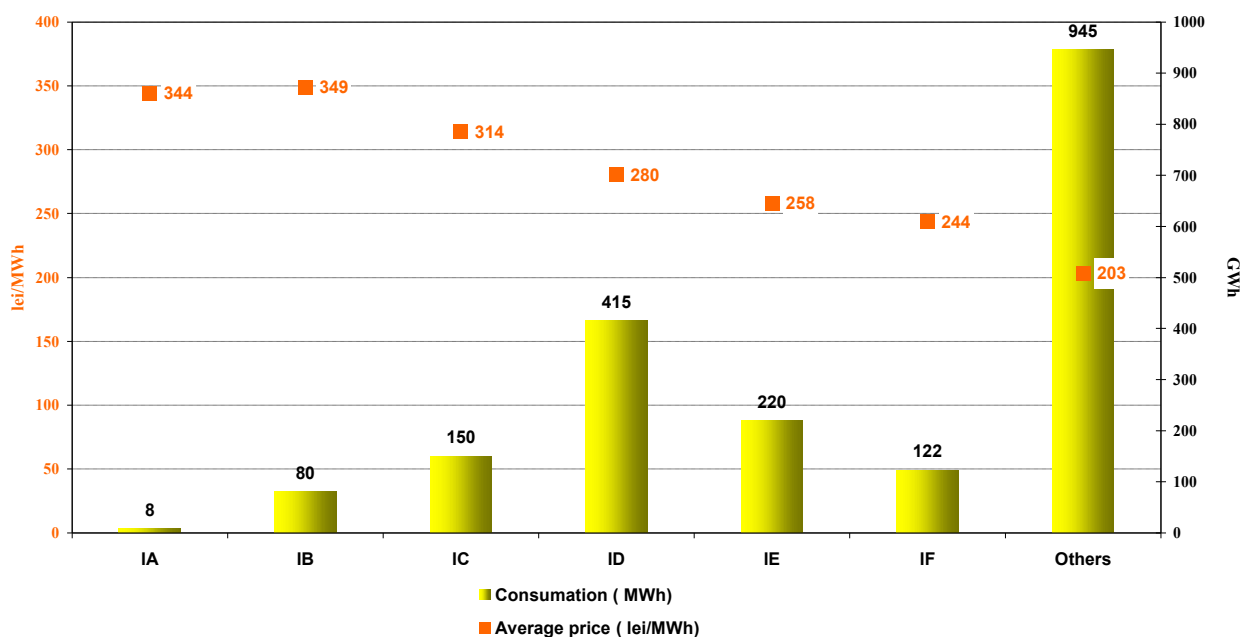
Average price and energy consumption on types of consumers applied on competitive market - July 2010 -
