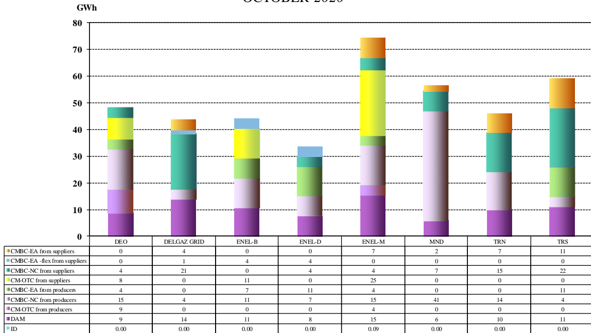
Structure of electricity acquisitions of distribution operators to cover distribution network losses - OCTOBER 2020 -
