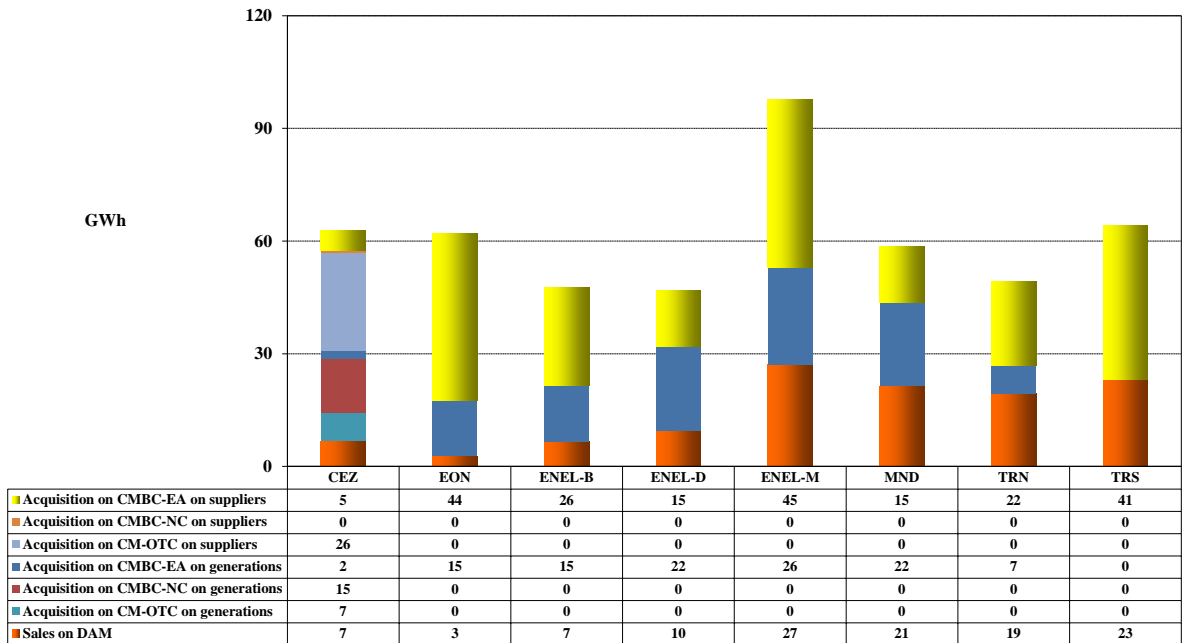
Electricity acquisition of distribution operators for covering the distribution losses OCTOBER 2016
