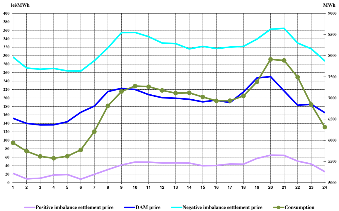
Hourly average settlement prices and internal consumption October 2016
