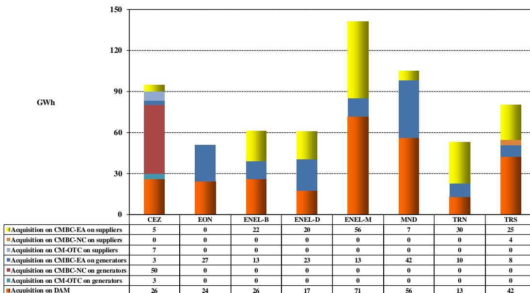
Electricity acquisition of distribution operators for covering the distribution losses February 2017
