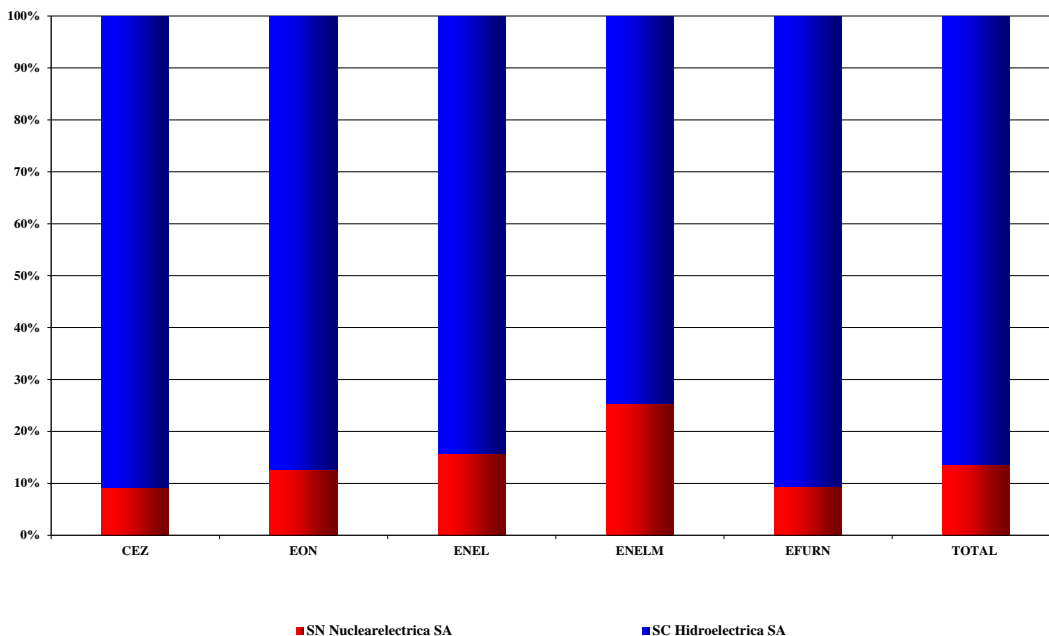
Electricity aquisition from main generators, on regulated contracts, of the suppliers of the last resort for delivering electricity to final consumers on regulated market MAY 2017
