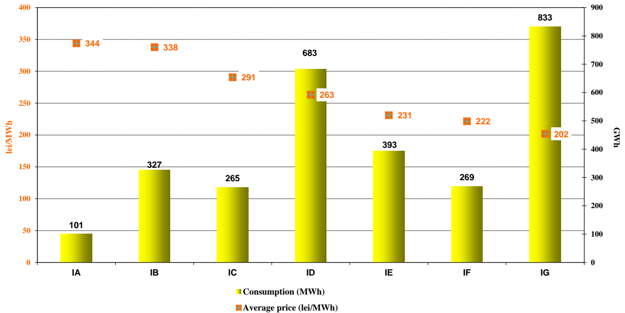
Average price and energy consumption for non-household customers' tranches on competitive segment of REM - May 2017 -
